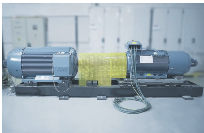
Test Bench at ABB's Service Center of Excellence
