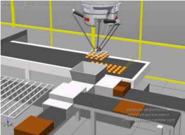
ABB Robot Studio Simulation With Multiple Station
