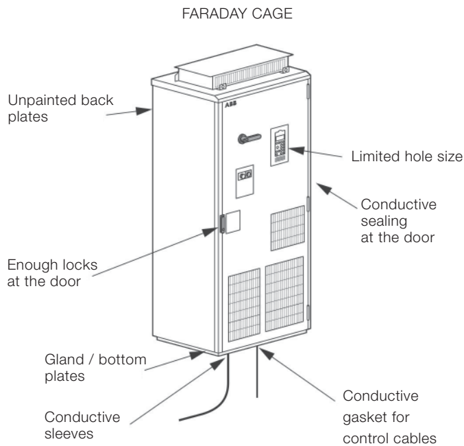
Figure 3-4 Typical enclosure aperture detail.
