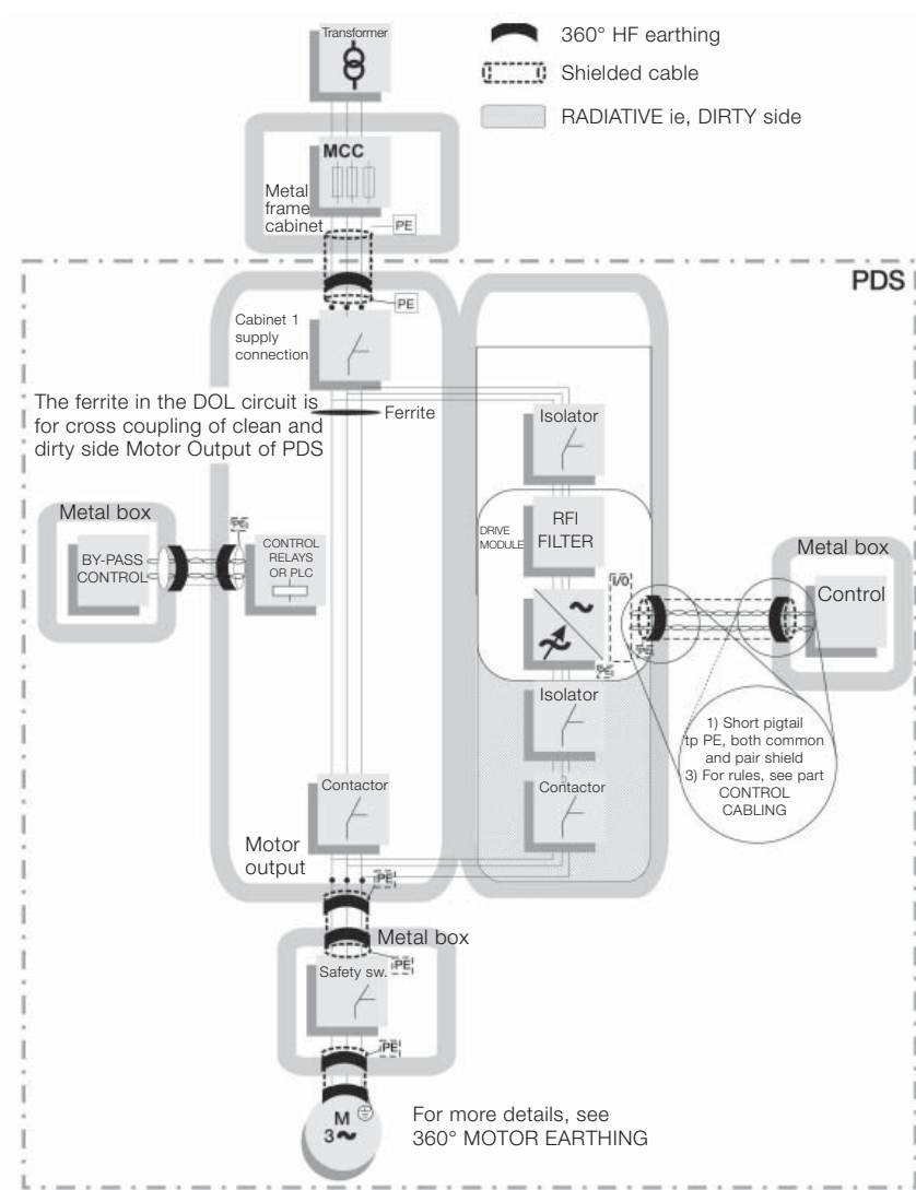
Figure 4-3 Basic scheme with by-pass.
