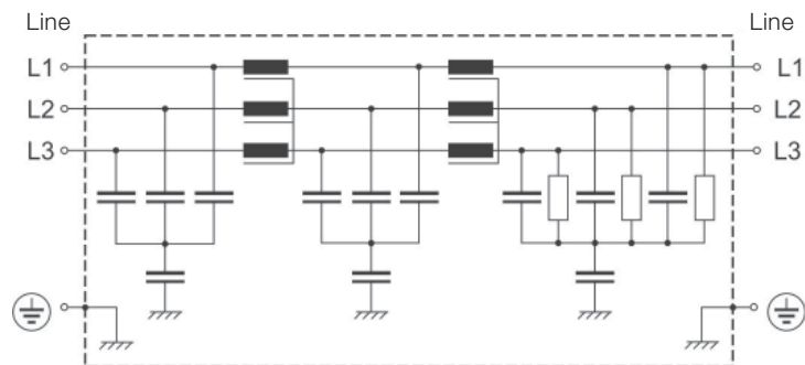
Figure 3-3 Example of filtering integrated in drive module.
