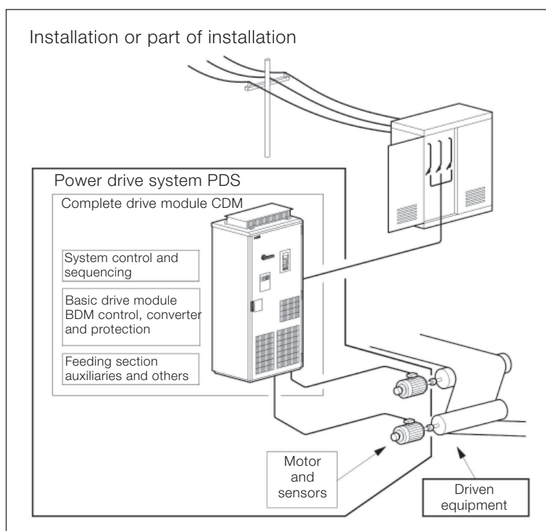
Figure 2-2 Abb reviations used in drives.
