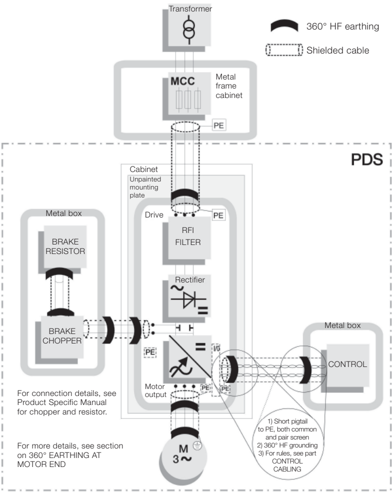
Figure 4-2 Typical PDS configuration.
