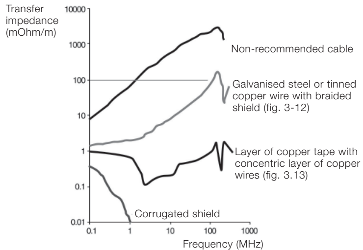
Figure 3-16 Transfer impedance for power cables.
